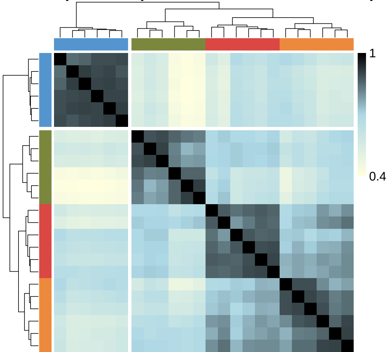
Compounds Spearman Hierarchical heatmap
